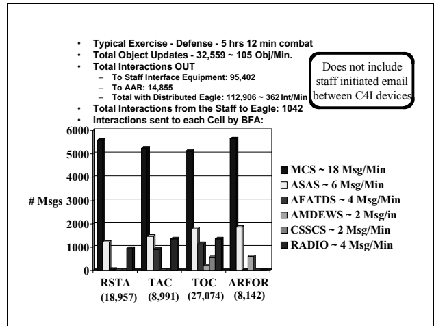
Message Traffic Analysis
