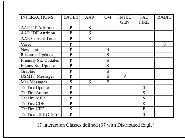
Federation Object Model
