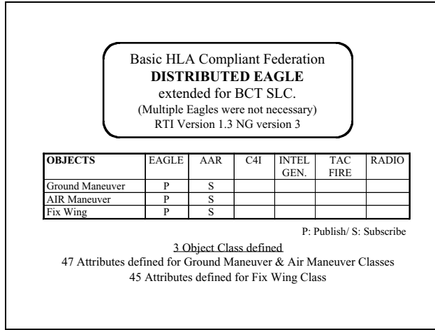
Federation Object Model
