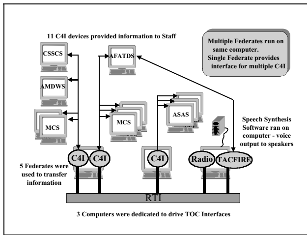
BCT Main TOC Configuration
