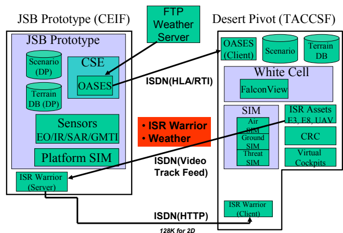
Figure 2: JDPE Event 1 Architecture and Data Flow
