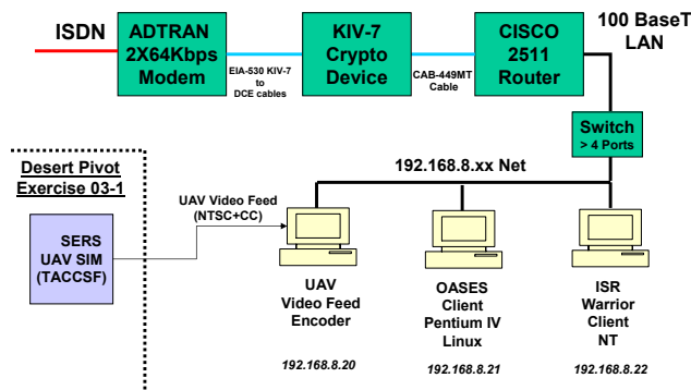
Figure 4: TACCSF Network and System Diagram for Event 1
