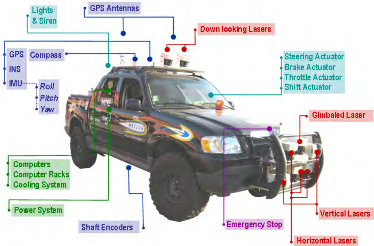
Figure 3: MITRE Meteor layout. Meteor has an array of COTS components. Positioning is by three GPS units, an INS unit and a compass on the roof. Four horizontal lasers detect road obstacles. Two vertically-mounted lasers provide terrain information. Two down-looking lasers detect small objects and negative spaces. A computer assembly is in the back seat.
