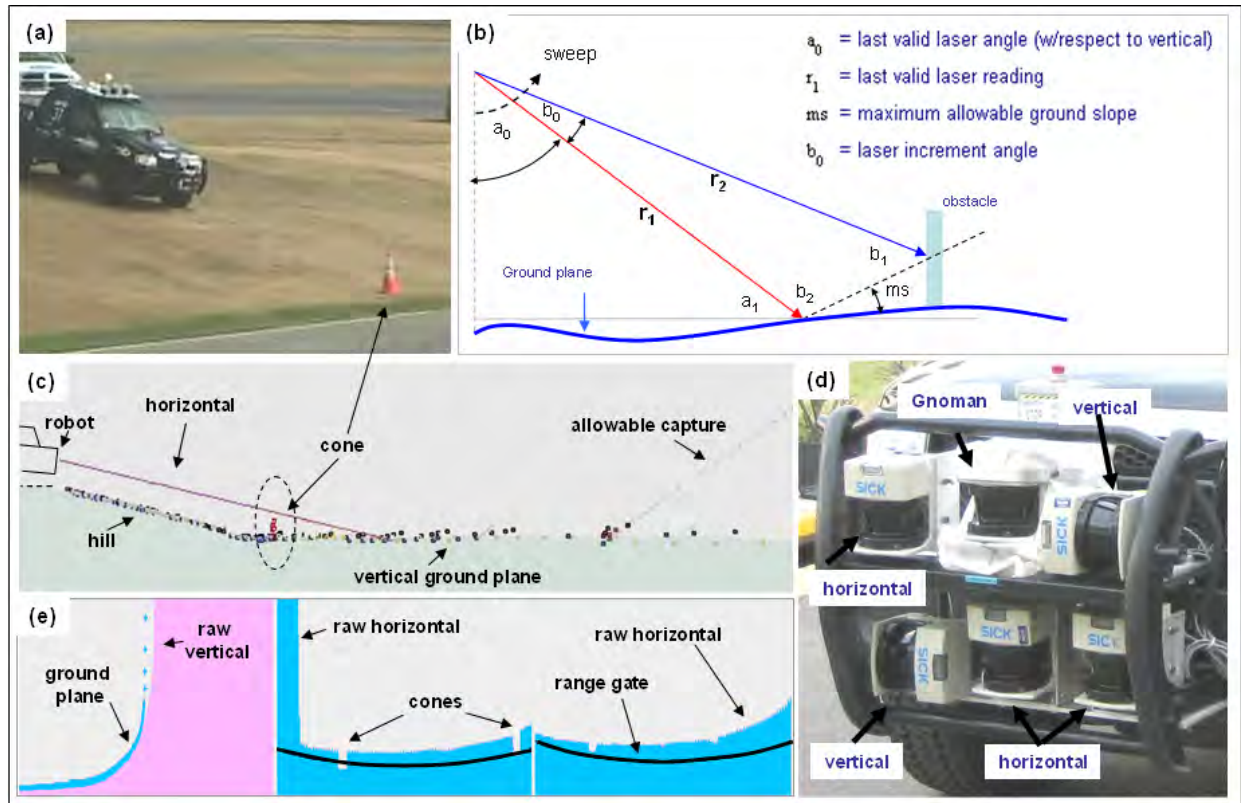
Figure 10: Vertical lasers. a) Meteor travels down a steep hill at the NQE. b) A slope filter removes obstacle readings from the vertical scan based on the slope change between readings to generate a ground plane estimate for range gating. c) A projection of the filtered ground plane just before Meteor begins to drive down the hill. Note the cone at the bottom of the hill (dotted ellipse) has been removed from the scan. d) The physical mounting of the lasers. A vertical laser collinear to the horizontal lasers it services. This alignment makes the range gate a simple geometric lookup in the vertical scan. e) Raw vertical laser scan (left pane, shaded) and projected ground plane (bowed line). Raw range scans from two horizontal lasers (center and left pane shaded). The crossing lines are the dynamic range gate. Note the cones on either side of the bottom of the hill are visible as gaps in the raw scans and are starting to show up as obstacles in two of the horizontals.
