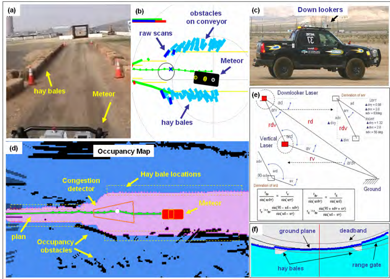
Figure 11: Down-looking. a) Meteor travels down the center of low-lying hay bales. b) Line segments generated by the down-looking lasers clearly show hay bales. Note Meteor correcting slightly right. c) Down-looking lasers mounted to the top of the roof rack. d) Occupancy map generated in the middle of the hay bales. The lane crosses the center image and narrows from right to left. Light areas indicate open space, dark segments are obstacles. Note that hay bales do not show up in the occupancy map. e) Like the vertical lasers, the down-looker ground plane filter is based on the Law of Sines. f) The raw output of a down-looking laser (shaded). The dark line riding on top of the raw readings is the horizontal ground plane. The hay bales are clearly seen in the scan. The ground plane shows Meteor slowly rolled to the left.
