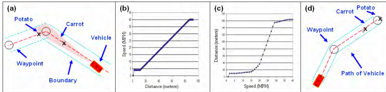
Figure 8: Carrot maneuvering. Steering stability is achieved using a “carrot” and “potato.” a) The carrot maintains its distance in front of the vehicle based on vehicle speed. Maximum vehicle speed is a function of path visibility and is determined by the potato. The potato defines visibility, the carrot follows the path, and the vehicle follows the carrot. b) A curve mapping the distance to the potato to maximum vehicle speed. c) A curve mapping actual vehicle speed to carrot distance. d) An example where a large carrot distance can cause a slight shaving of the defined route.
