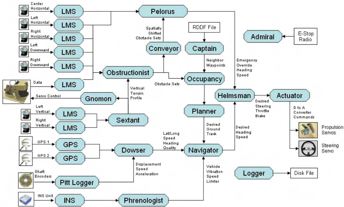
Figure 5: Software architecture implementation. An agent-based architecture converts raw sensor information into voltages to drive the robot. “Lookouts” convert raw sensor data into system messages. “Watch Officers” turn raw information into information like obstacles and position. The “Captain” takes the RDDF and defines the next achievable point and the lane in which the vehicle can operate. The “Planner” uses the lane and obstacles generated by the lasers to generate a plan. The “Navigator” determines desired speed and direction based on the plan and the vehicle’s state. The “Helmsman” converts the speed and direction into commands that cause the EMC system to produce motion. The “Admiral” monitors the E-Stop radio and gives the master go signal.
