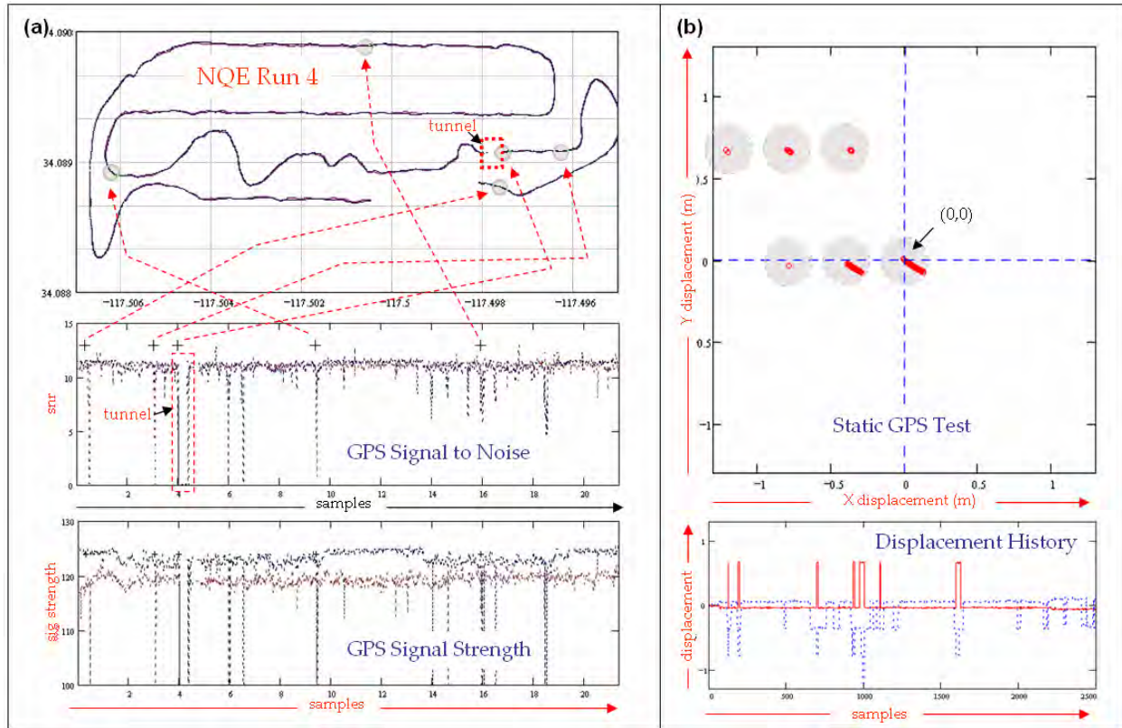
Figure 7: GPS verification. GPS reliability is determined by assessing signal strength and signal-to-noise ratio reported by GPS units. If the ratios drop below a set threshold, their reported positions are not trusted and Meteor is guided by a dead reckoning model. a) Signal-to-noise ratio and signal strength plots during a run at the NQE. Circles correspond to selected points on the plots. Note the complete drop out inside the tunnel. b) 2500 GPS readings taken while the robot was stopped during testing at the NQE. Note the apparent spatial periodicity implying multipath. Below is the same series as a function of time and displacement.
