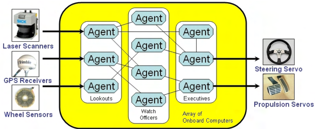
Figure 4: Basic agent makeup. Lookout agents manage sensors and convert raw sensor information into system messages. Watch Officers process and fuse sensor data from Lookouts into higher order information. Executives use Watch Officer products to make decisions that ultimately control the actions of the Meteor.
