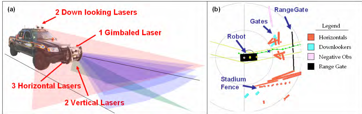
Figure 9: Sensor types. a) Meteor carries four classes of laser sensors. Three fixed horizontal lasers mounted at slightly different angles detect obstacles directly in front of the vehicle. A gimbaled horizontal laser tracks the horizon providing the greatest sensing distance. Two vertically-mounted lasers detect road terrain and provide dynamic range gating to the horizontal lasers. Two down-looking lasers detect small ground obstacles and negative terrain. b) Line objects generated by each laser are displayed during testing. This is a view of Meteor as it is about to pass through the first gate at the NQE.
