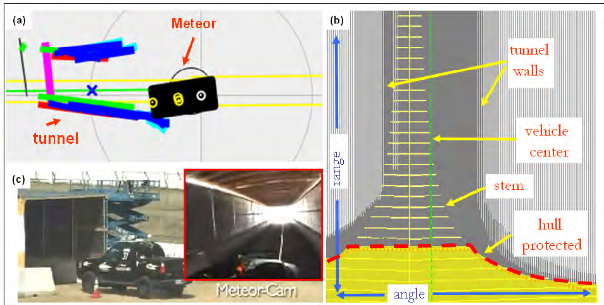
Figure 13: Reactive. a) Laser line obstacles generated as the vehicle passes through the tunnel. A mismatch in heading shows the vehicle thinking it is about to collide on the left. b) Instantaneous lasers represented in polar coordinates with respect to vehicle centerline. The vehicle finds a steering correction angle that will guide the vehicle reactively and avoid obstacles. This representation shows the vehicle is closer to the right wall. c) The vehicle as it enters the tunnel at the NQE. The tunnel is lined with metal sheets to block all GPS signals.
