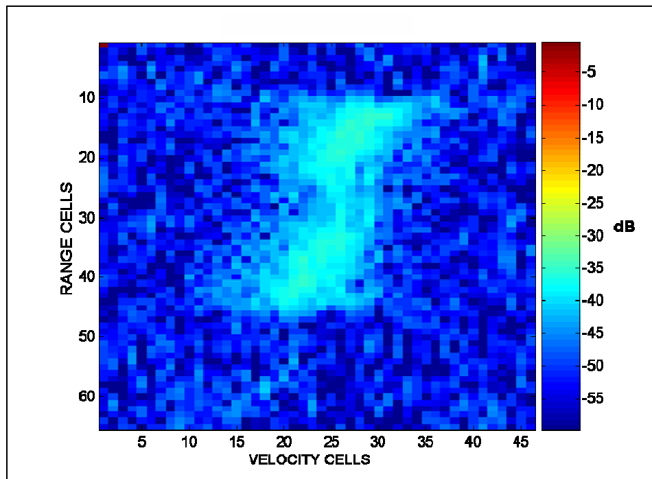
Figure 8. Improvement in Contrast in the Phase Image due to Clutter Cancellation (Target Auto-detected)
