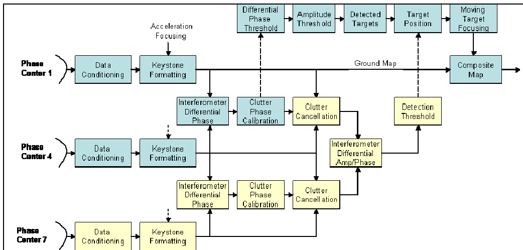
Figure 7. Block Diagram of Moving Target Detection and Tracking Using Multiple Phase Centers
