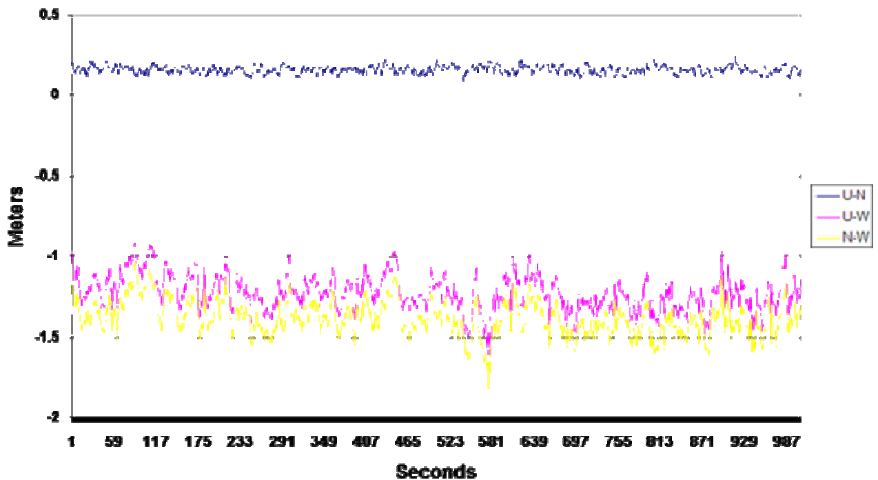
Figure 5. Differential Group Delays Measured Between Channels of a Commercial GPS C/A-code Receiver Employing Three Early-Late Correlator Spacings.
